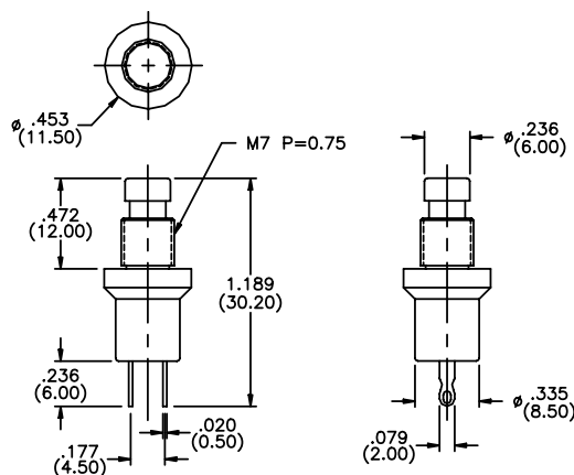
MECHANICAL OUTLINE
