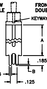
FRONT VIEW DOUBLE POLE
